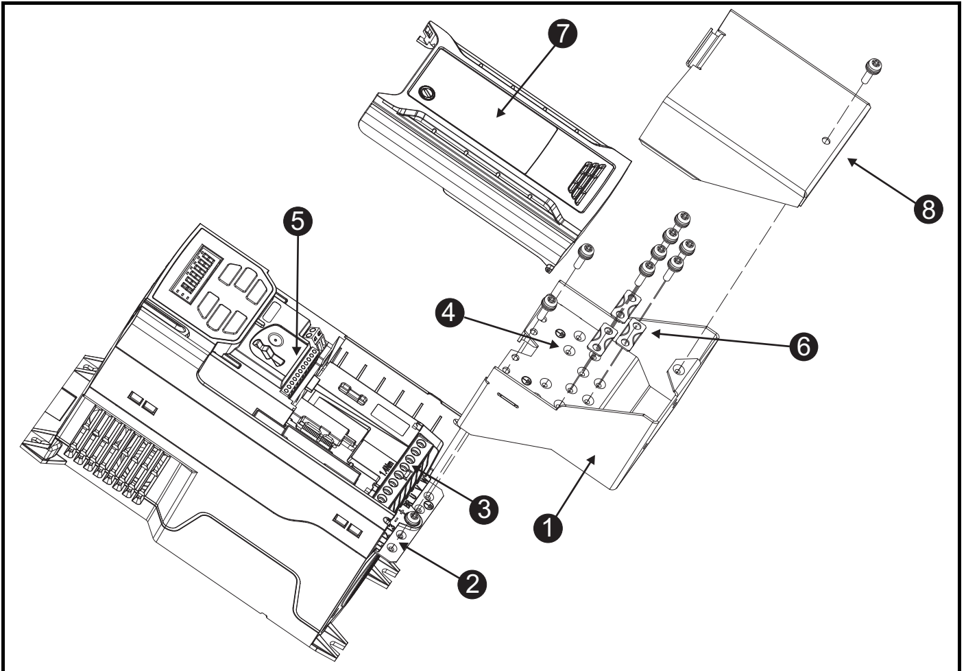
Figure 3-3 Installation of conduit connection box
