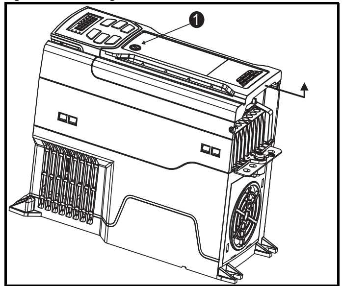
Figure 3-1 Removing the drive terminal cover
