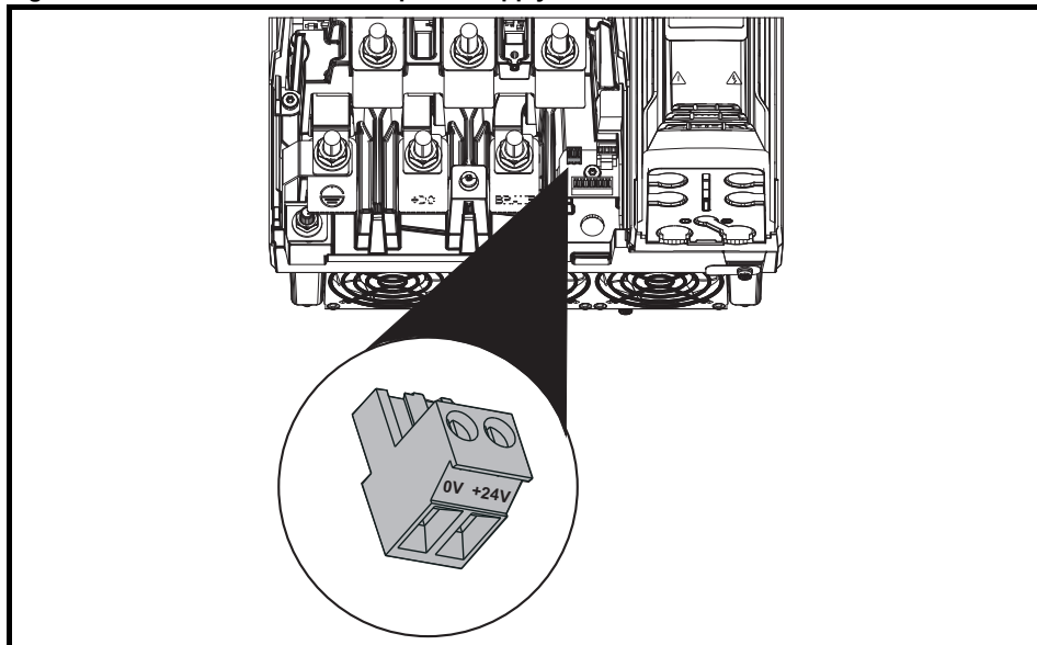
Figure 4-7 Location of the 24 Vdc power supply connection on size 8 to 10
