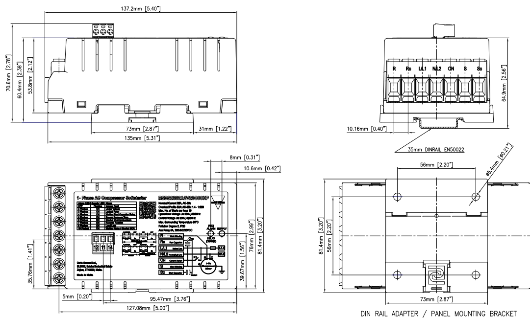
Fig. 1 RSBS2332A2V23C00HP
