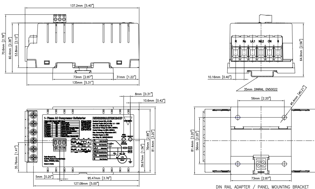
Fig. 2 RSBS2332A2V23C..HP
