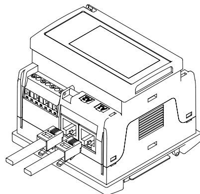
Fig. 19 RJ12 connections
